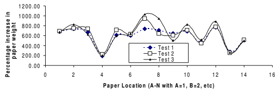
Figure 9 Typical repeatability coverage trials for 30s
