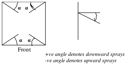
Figure 5 Orientations and angles of the fine spray swirl atomisers and the Hughes safety shower nozzles in the test chamber
