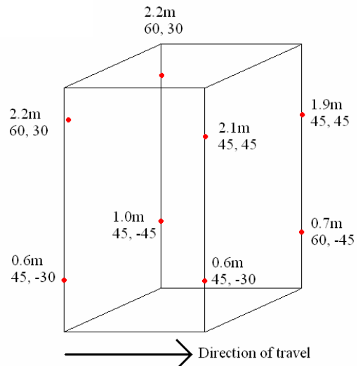
Figure 6 A fine spray configuration for effective total coverage.
