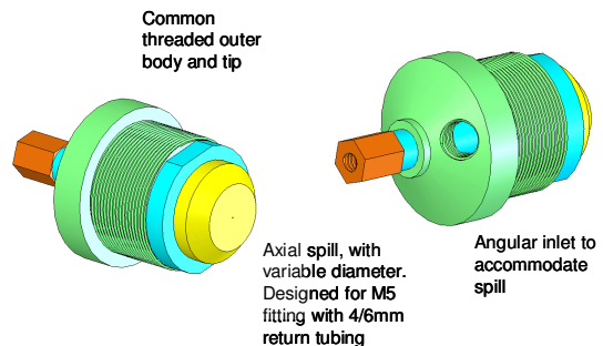
Figure 4 High pressure, low flow rate swirl atomiser with 0.3mm exit orifice
